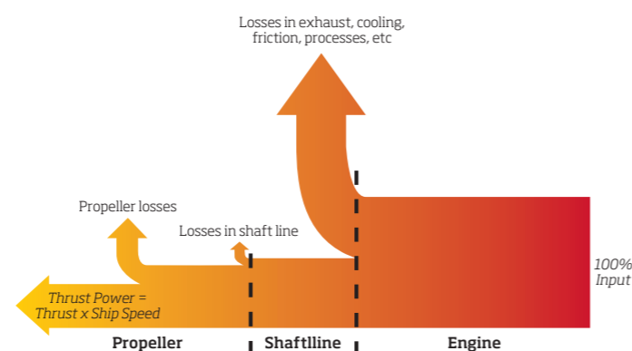
Figure 2.1 Typical power utilisation in a tanker or bulk carrier
