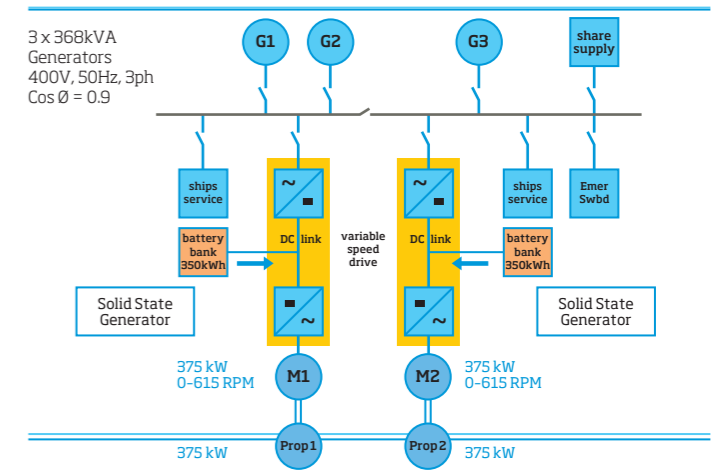
Serial hybrid system
