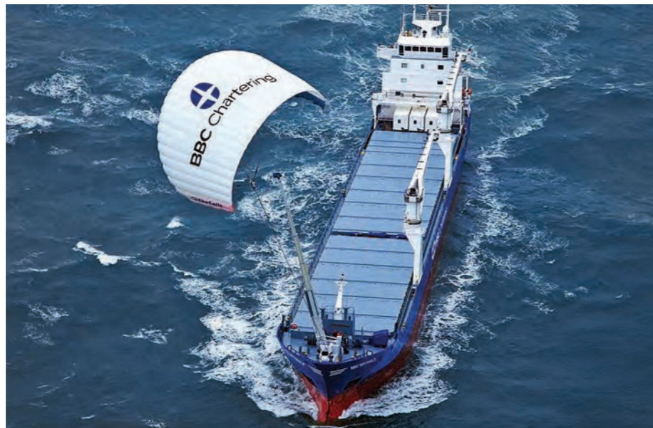
Figure 3.15 Application of a kite to assist propulsion © Sky Sails
