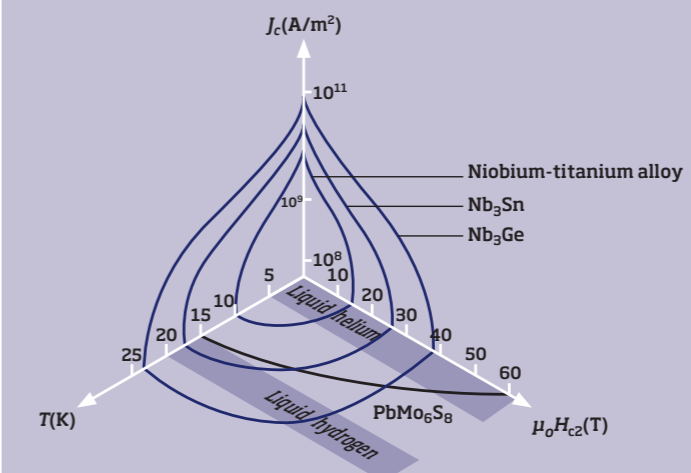
Typical current, field and temperature dependencies of superconductivity.
