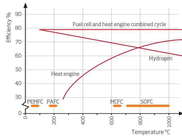
Figure 3.10 Theoretical heat engine and fuel cell efficiencies [Larminie and Dicks 2000]
